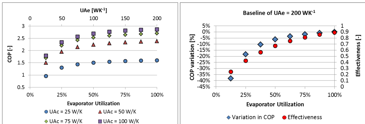
Figure 3: Left: Influence of evaporator utilization on appliance COP for various UA_c values. Right: Reduction in COP with reducing evaporator utilization and corresponding evaporator effectiveness (Janna, 2000), data based on the average COP resulting for the various UA_c values presented in the left figure. Calculations are based on using R-290 as refrigerant, T_a = 25 \text{ °C} , T_i = 2 \text{ °C} , V = 350 \text{ m}^3\text{h}^{-1} , \eta_i = 0.45 , Q = 175 \text{ W} , Q_c = 350 \text{ W} and UA_e = 200 \text{ WK}^{-1} .
