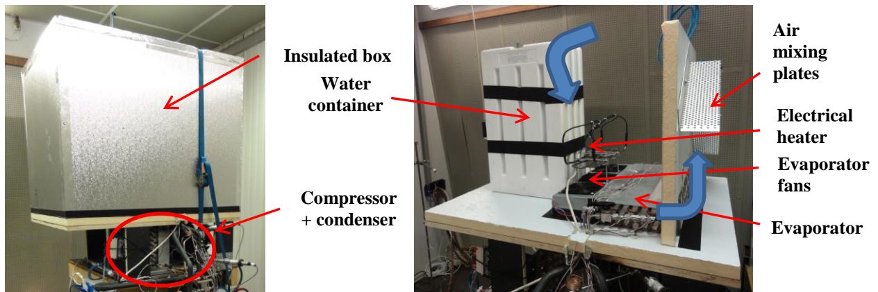
Figure 4: Test rig used to evaluate control strategy “Left: With insulated box, Right: After removal of insulated box, Blue arrows indicating internal air flow direction”
