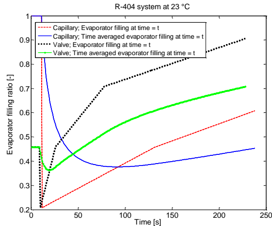
Figure 9: Momentary and time averaged evaporator filling obtained with the capillary and with optimized opening profile of the expansion valve.
