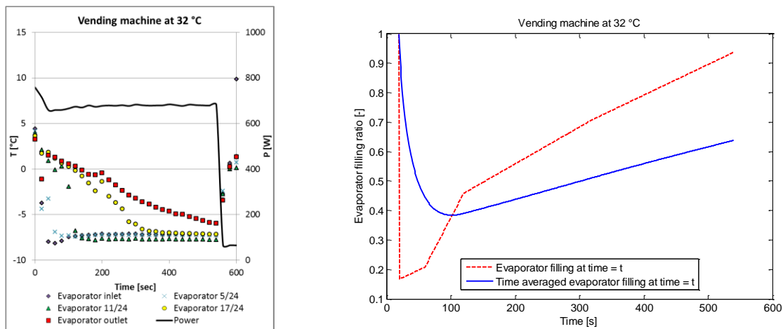
Figure 1: Operating cycle of R-404A based vending machine during steady state operation at an ambient temperature of 32 °C, where time t = 0 s indicates the activation of the compressor. Left: Measured evaporator tube temperatures, in which a steep drop in temperature indicates the time at which the two phase flow front approaches the specific position. Right: Momentary (FR) and time averaged ( \overline{FR} ) evaporator filling during the operating cycle estimated from the temperature readings.
