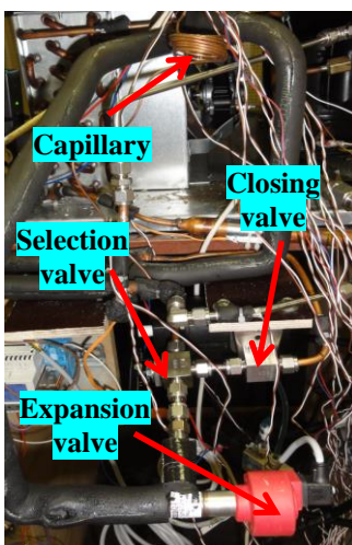
Figure 5: R-744 system
