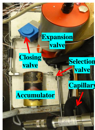
Figure 6: R-404A system
