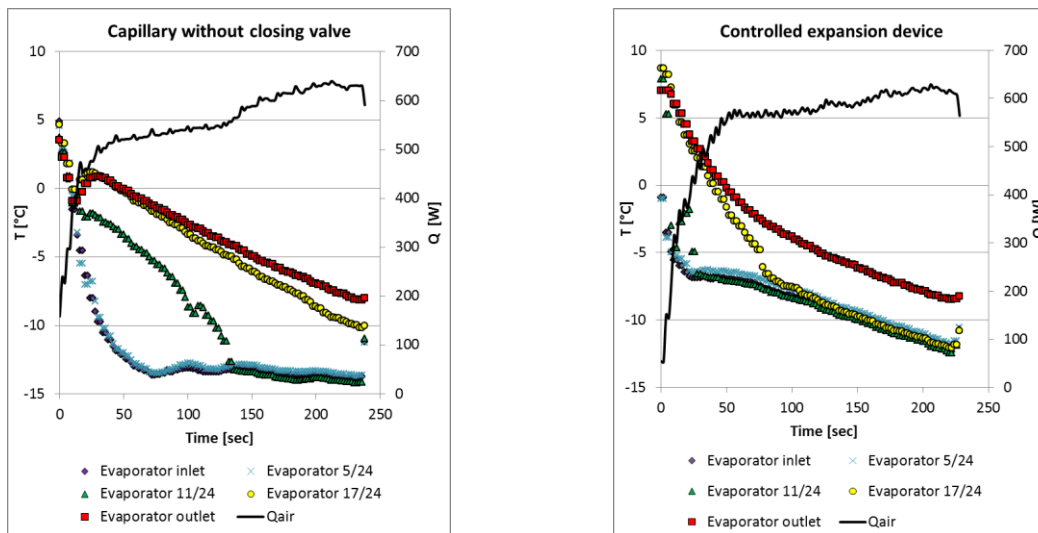
Figure 8: Evaporator filling of R-404A system during compressor on period at an ambient of 23 \text{ }^\circ\text{C} . “Left: operation with capillary. Right: Operation with controlled expansion valve using optimized linear opening profile”
