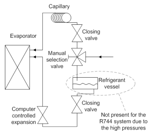
Figure 7: Dual expansion set-up
